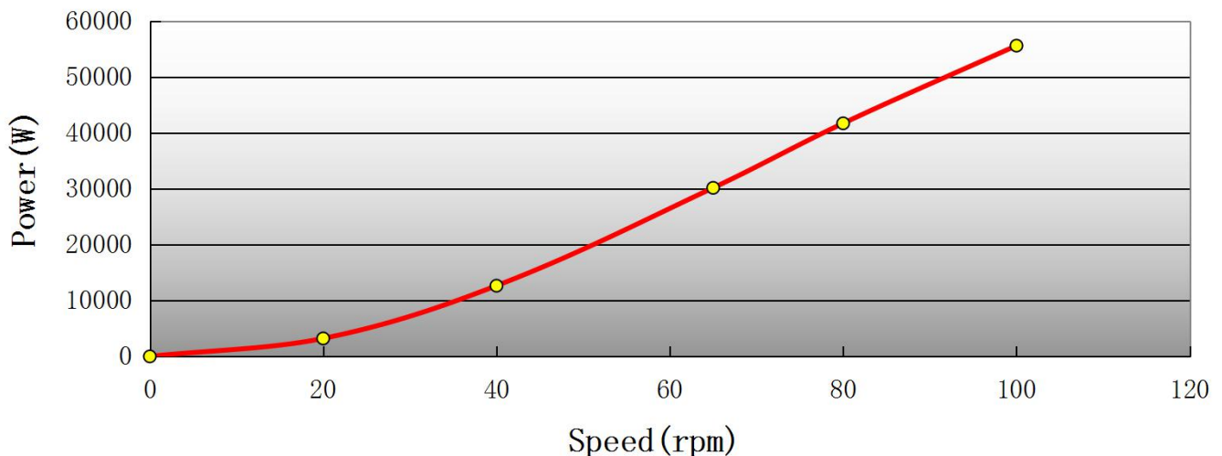
Load Power curve
