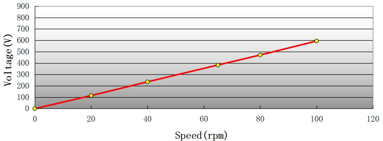
Open-Circuit Voltage Curve
