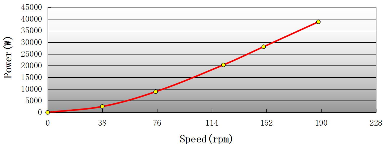
Load Power curve
